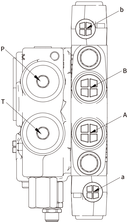
FS04/09/12-不带液压锁
