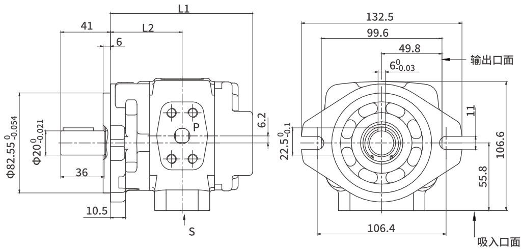
HG0-※-01R-VPC(平键轴)
