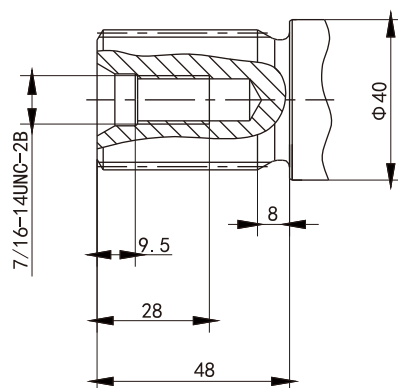
T 花键轴 1 3/8" 21T 16/32DP
