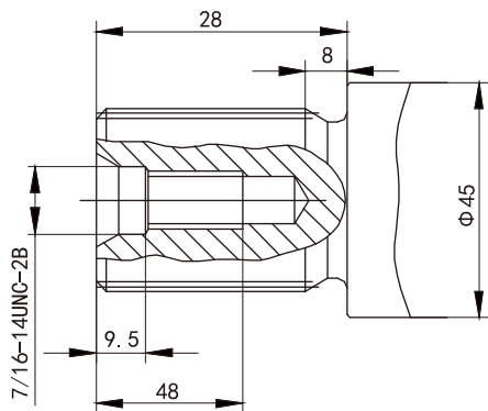
U 花键轴 1 3/8" 21T 16/32DP
