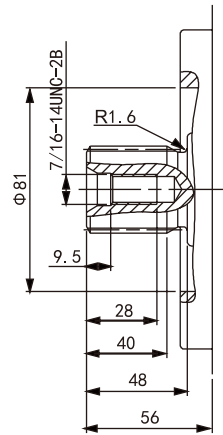
T 花键轴 1 3/8 in 21T 16/32DP
