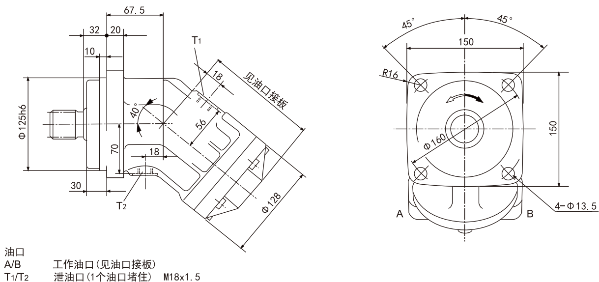
HA2FM 56/63
