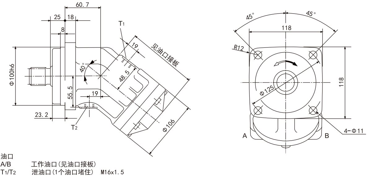
HA2FM 23/28/32
