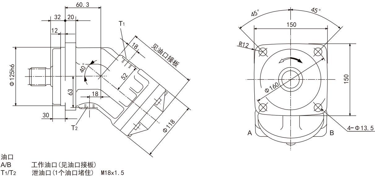
HA2FM 45
