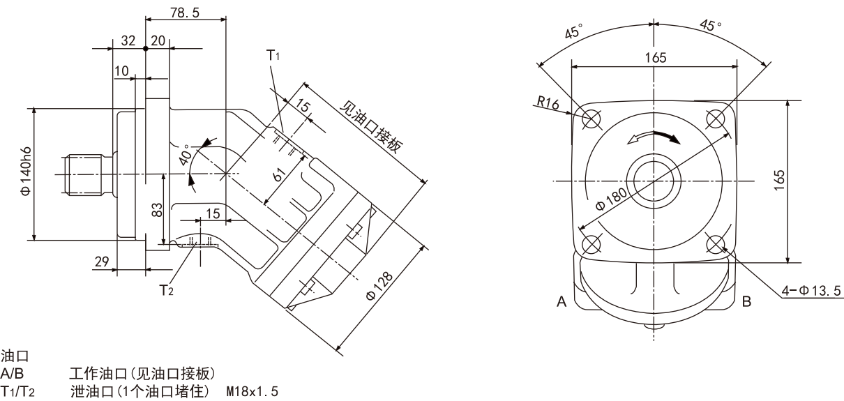
HA2FM 80/90
